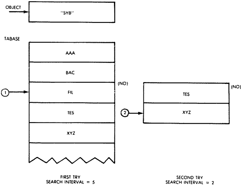
Fig. 9.19: A Binary Search
